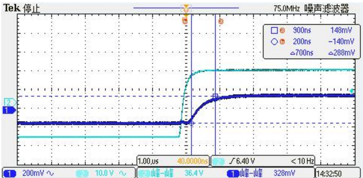
Fig.2 the step response time of STK-HD/P1/x current sensors. The light blue is primary current, while the dark blue is output signal of current sensor. The step response time is less than 1.0 \mu s.
